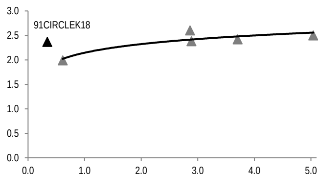
CIRCLEK 22 (THIE-28) – Relative Value AxV vs. Sobretasa (%)
